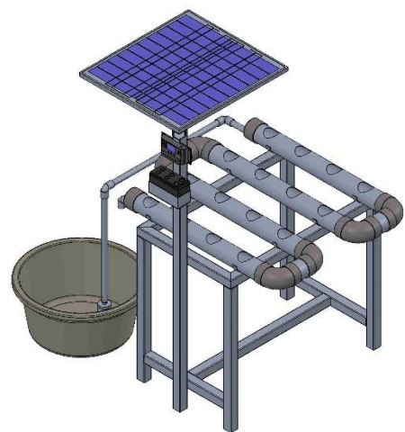
Tampak Isometri
