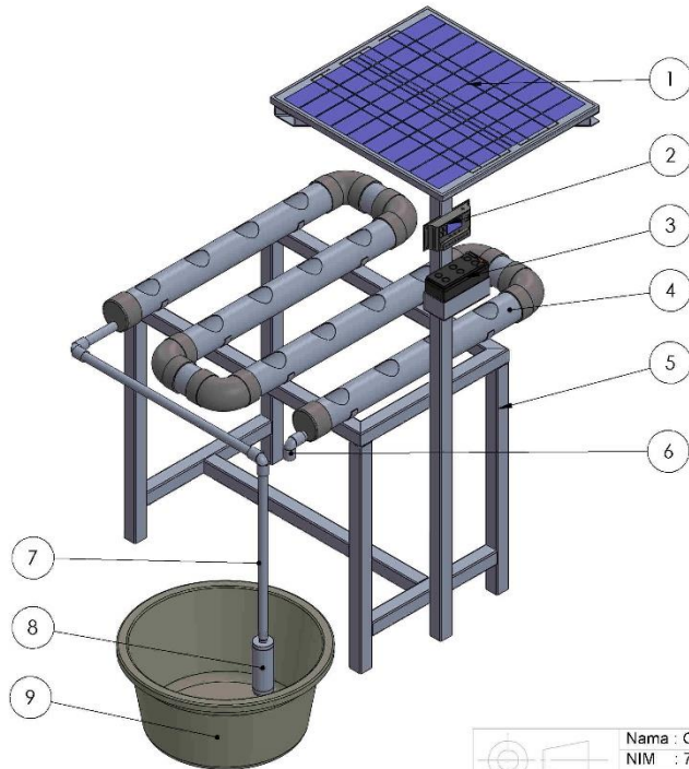
Tampak Isometri
